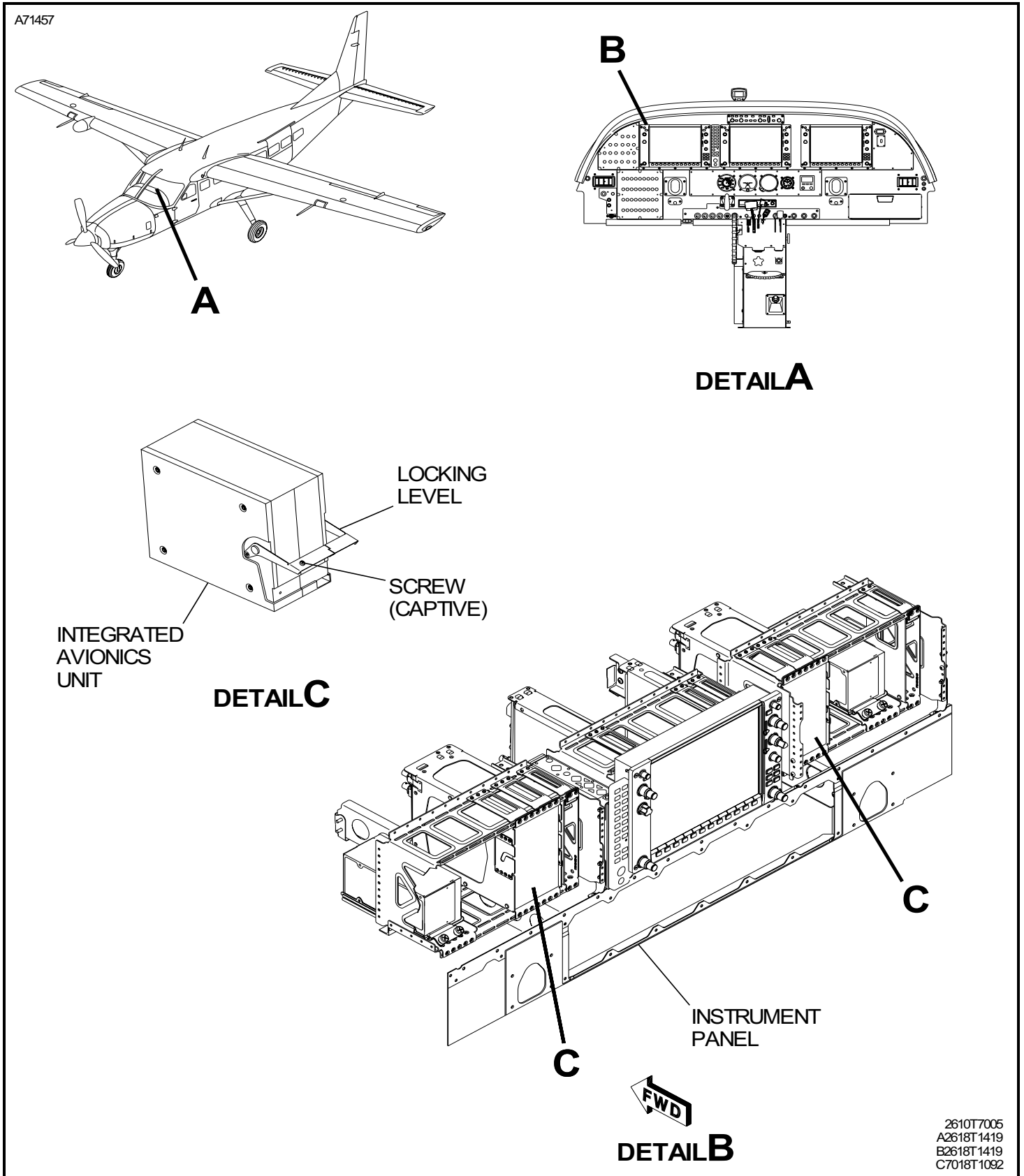
Figure 401 : Sheet 1 : GIA 63 Integrated Avionics Unit Installation
